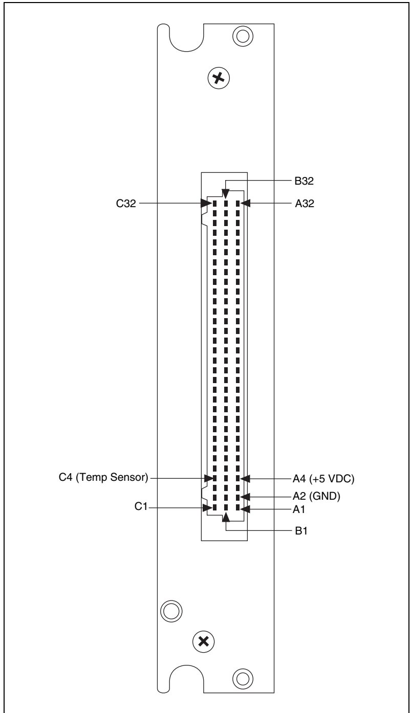
Figure 1. SCXI-1320 Front Connector Pin Assignments
