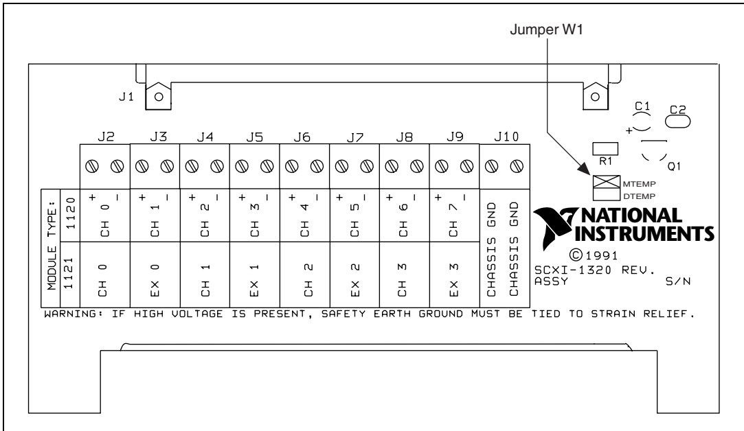
Figure 2. Location of Jumper W1 on the SCXI-1320 Terminal Block
